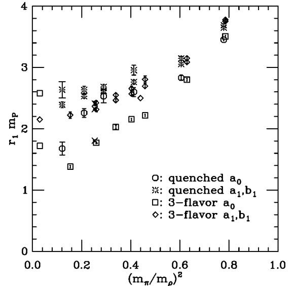
FIG. 15. P-wave meson masses in units of r_1 . The bursts are the quenched pseudovector mesons ( a_1 and b_1 ), and the diamonds the full QCD pseudovectors. Where the difference is significant the 1^{+-} ( b_1 ) state is heavier than the 1^{2+} state. The octagons are the quenched scalar ( a_0 ), and the squares the full QCD scalar. Crosses are the two flavor results. The diamond at the physical value of (m_{\pi}/m_{\rho})^2 is the experimental a_1 and b_1 mass, and the two squares are experimental 0^{2+} ( a_0 ) masses.
