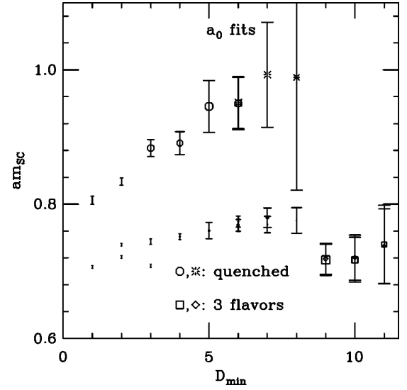
FIG. 14. Fitted masses for the scalar ( a_0 ) meson with quark mass am_{u,d} = 0.03 as a function of the minimum distance included in the fit. In this plot the symbol size indicates the confidence level of the fit, with the symbol size used in the legend corresponding to 50%. Here the octagons are quenched results using two 0^{-+} (pion) states and one 0^{2+} ( a_0 ) state, while the bursts are quenched results with one state of each parity. The squares and diamonds are 2+1 flavor results using two and one 0^{-+} states respectively.
